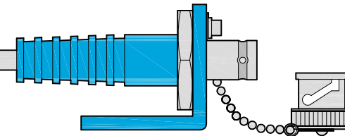
BNC Connector with Dustcap and 90° Bracket
