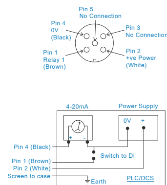
Connection Details Top & Bottom Connector
